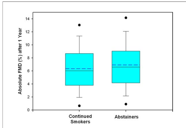
Figure 1 Absolute FMD Values 1 Year After Quit Date, Expressed as Percentages
